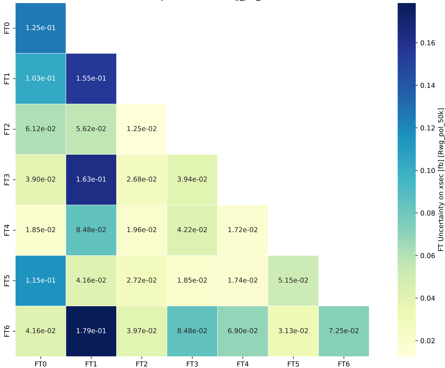
FT Uncertainty on xsec [fb] [Rwg_pol_50k]
